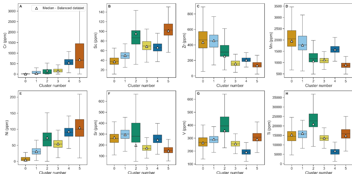
Supplementary Figure 25. Clustering data imbalance. Boxplots show the distribution of trace-element concentrations for the six clusters obtained from the K-means model fitted to the full dataset (LA-ICP-MS map pixels and single-spot analyses). Elements shown are Cr, Sc, Zr, Mn, Ni, Sr, V, and Ti, similarly to Fig. 8A-H. White triangles indicate the median composition of the corresponding clusters produced by an independent K-means model fitted to a balanced dataset composed of all single-spot analyses ( n = 316 ) and a random downsample of 1000 map pixels. The clusters from the balanced model were matched to the reference full-dataset clusters by nearest-centroid distance in the scaled eight-element compositional space. The close agreement between the balanced-cluster medians and the full-dataset boxplots indicates that the main six-cluster structure is reproduced when clustering is rerun on a dataset less dominated by map pixels, supporting the robustness of the solution to the pixel:spot imbalance.
