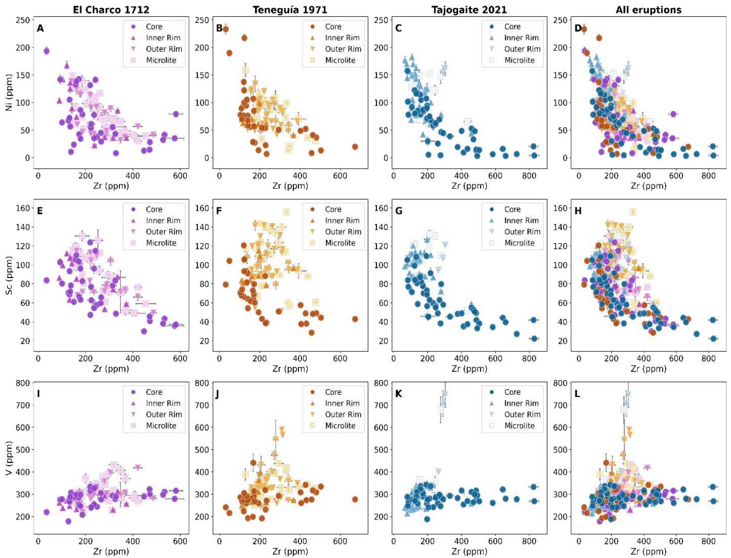
Supplementary Figure 5. Cpx compatible TE composition (Ni, Sc, V). Clinopyroxene trace element bivariate plots of (A-D) Ni (E-H) Sc and (I-L) V vs Zr. Each column corresponds to a different eruption, as indicated by the column titles, with the final column showing data from all eruptions combined. Each symbol represents a different clinopyroxene textural position. Error bars indicate the internal 2SE analytical uncertainty.
