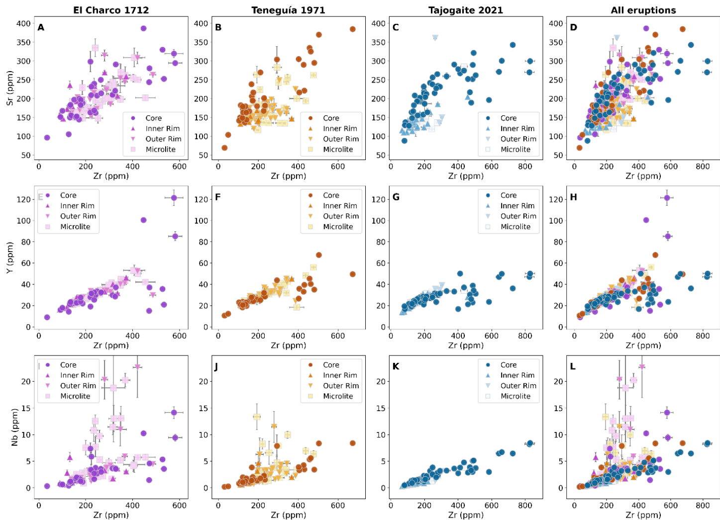
Supplementary Figure 6. Cpx incompatible TE composition (Sr, Y, Nb). Clinopyroxene trace element bivariate plots of (A-D) Sr (E-H) Y and (I-L) Nb vs Zr. Each column corresponds to a different eruption, as indicated by the column titles, with the final column showing data from all eruptions combined. Each symbol represents a different clinopyroxene textural position. Error bars indicate the internal 2SE analytical uncertainty.
