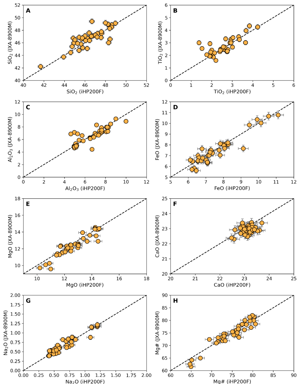
Supplementary Figure 23. EMPA Comparison Tajogaite 2021. Comparison of major and minor element data for samples from Tajogaite 2021 collected with the iHP200F microprobe in Madrid and the old JXA-8900M microprobe in Madrid. Error bars indicate 2\sigma uncertainties derived from EMPA counting statistics.
