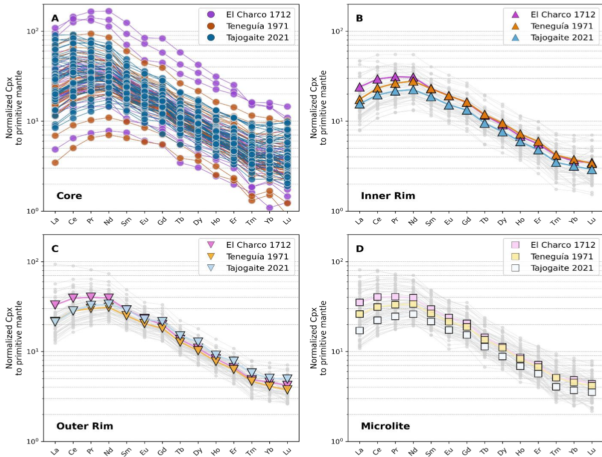
Supplementary Figure 10. Texture-grouped cpx REE patterns. Rare earth element (REE) patterns of clinopyroxene, normalized to the composition of primitive mantle 26 . REE patterns of cores are shown as individual data, whereas for inner rims, outer rims, and microlites we show the average for each eruption, with individual patterns displayed in light grey.
