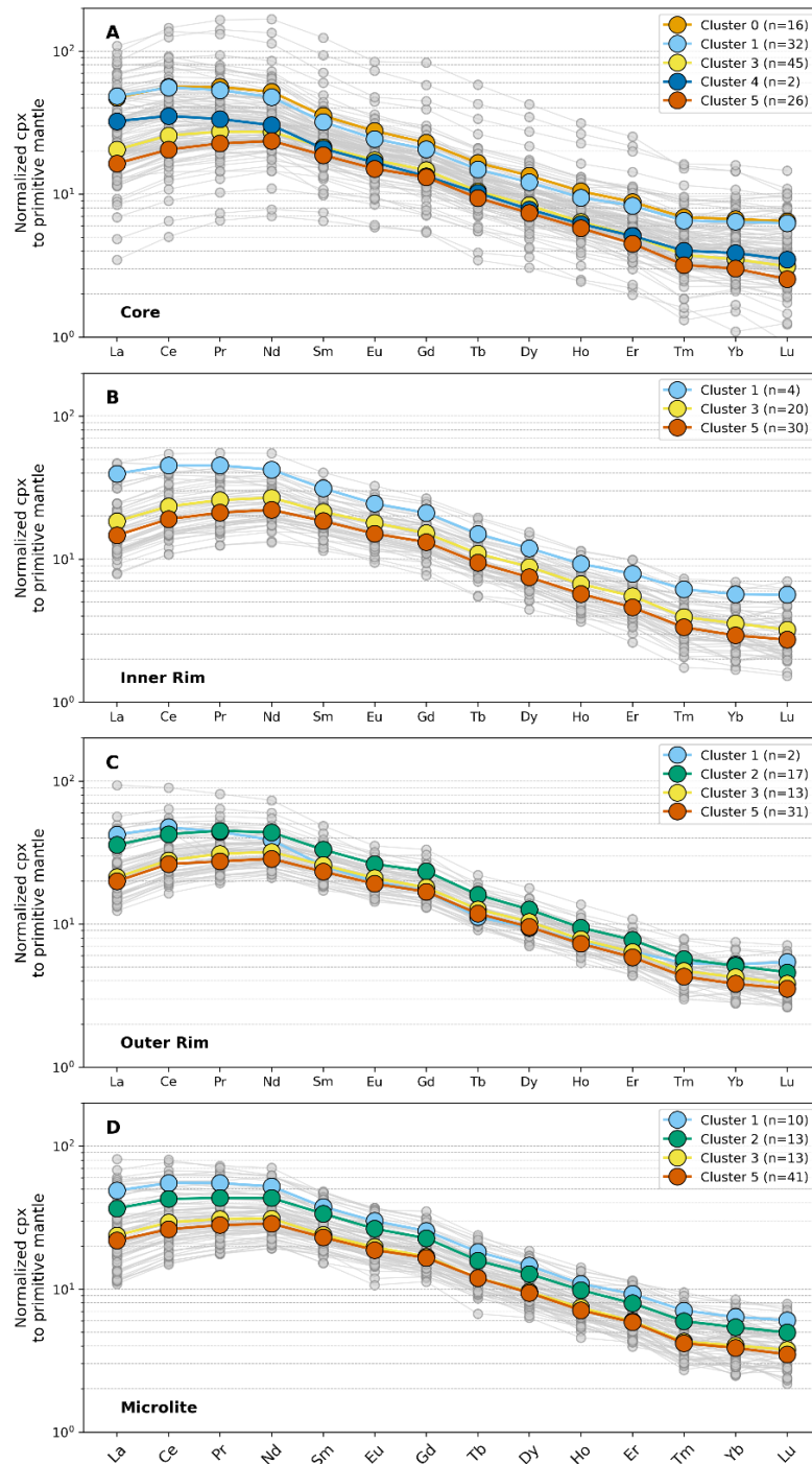
Supplementary Figure 16. Cluster-colored cpx REE patterns. Trace element patterns are color-coded based on clusters. Grey lines and points represent individual measurements, while colored lines show the average for each cluster group. Each panel corresponds to a specific textural position: (A) core (B) inner rim (C) outer rim and (D) microlite.
