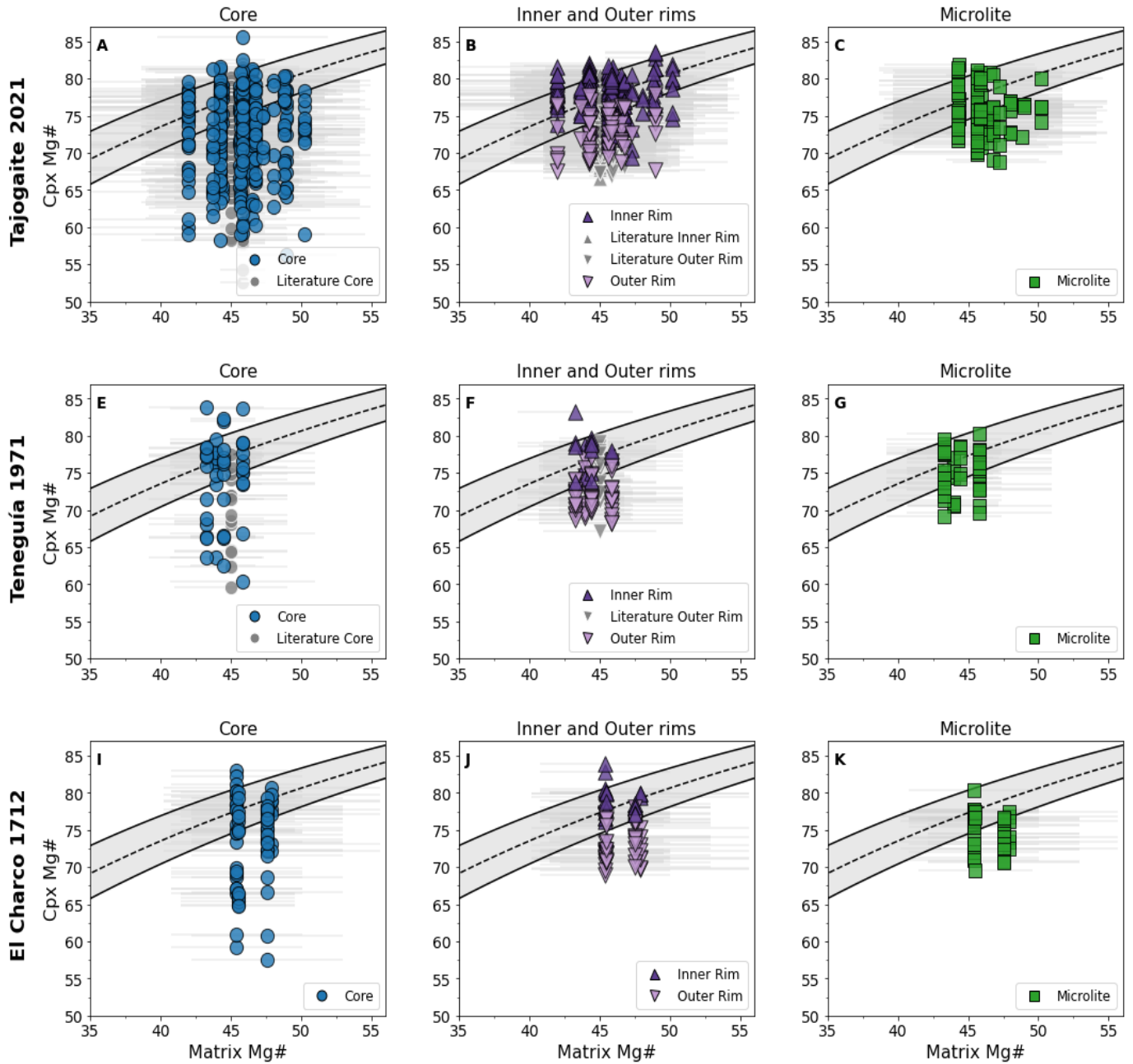
Supplementary Figure 2. Cpx – melt equilibrium. Matrix Mg# vs clinopyroxene Mg# for (A-C) Tajogaite 2021 (E-G) Teneguía 1971 and (I-K) El Charco 1712. Each symbol and color represent a different textural position (Core, Inner and Outer rims, Microlites, and Cpx inclusions), as indicated in the legend. Gray symbols correspond to literature data 22–24 . Inner rim and microlite compositions from the 2021 Tajogaite eruption are from Ubide et al. (2023) 15 . The gray field in each panel indicates the KD(Fe-Mg)_{cpx-melt} of 0.28 \pm 0.08 25 , which is used to assess major element equilibrium between clinopyroxene and the matrix composition. Horizontal error bars reflect the matrix Mg# 2 \sigma variability.
