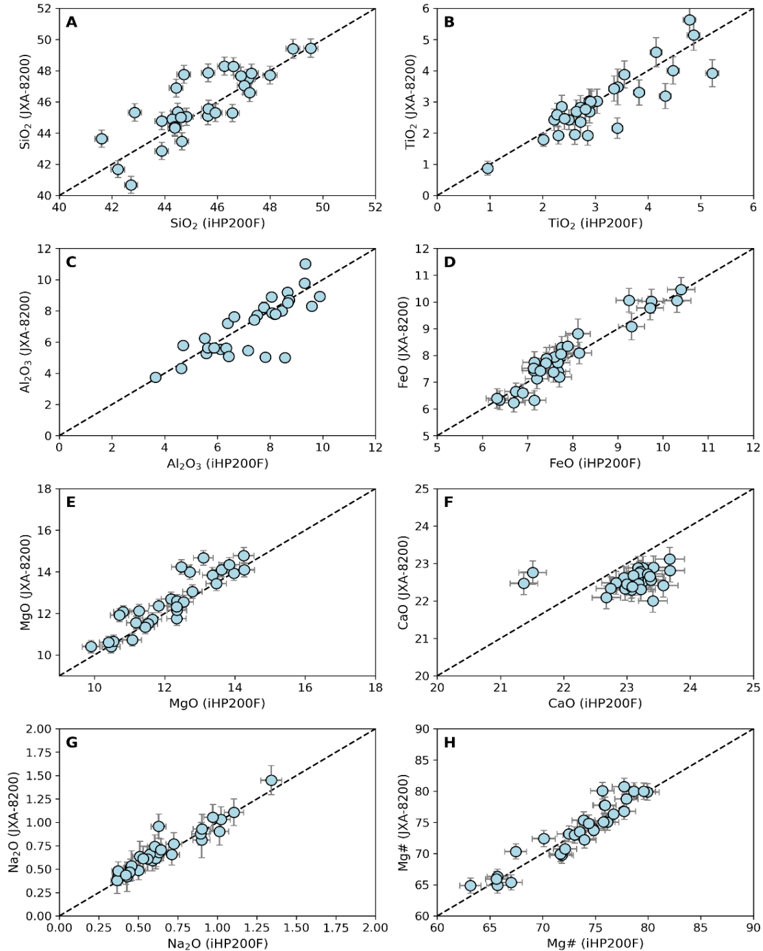
Supplementary Figure 22. EMPA Comparison El Charco 1712. Comparison of major and minor element data for samples from El Charco 1712 collected with the new iHP200F microprobe in Madrid and JXA-8200 microprobe in Huelva. Error bars indicate 2\sigma uncertainties derived from EMPA counting statistics.
