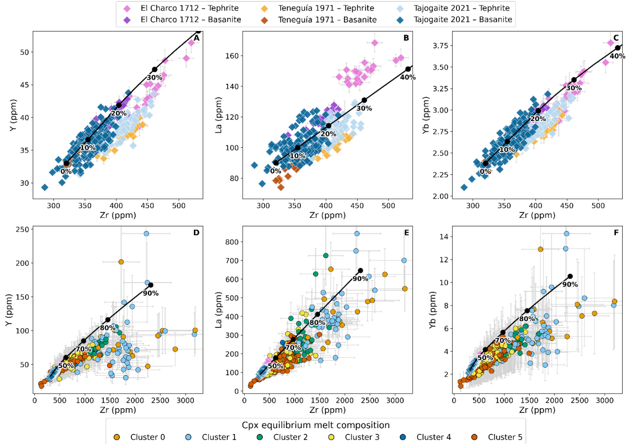
Supplementary Figure 19. Equilibrium melt composition and FC model. (A–C) Trace element composition of the matrix and FC results from the thermodynamic-based MAGEMin model. Each black filled circle represents 10% increments of fractionation starting from 100% melt phase. Note that the tephrite compositions for each eruption can be reproduced by ~10-20% fractionation from a basanite composition of the same eruption. (D–F) Reconstructed clinopyroxene equilibrium melt compositions, colored according to clustering. The black line represents the thermodynamic-based MAGEMin FC model. Note that Clusters 0 and 1 compositions are consistent with 80–90% fractionation.
