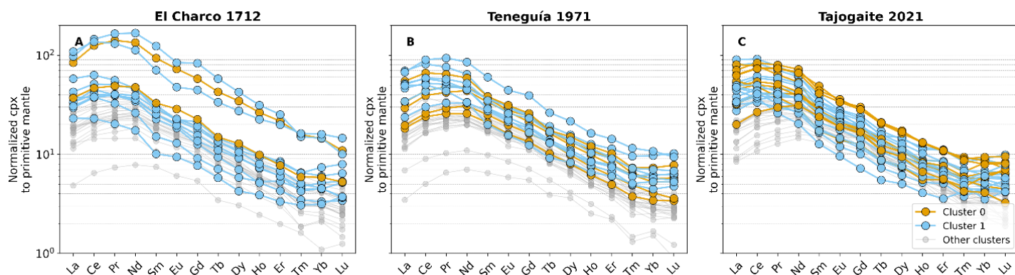
Supplementary Figure 17. Evolved cpx REE patterns. Trace element pattern of evolved clinopyroxene cores belonging to Cluster 0 and 1. These compositions are the most differentiated, with patterns showing an enrichment in heavy REE elements Tm, Yb and Lu, typical of phonolite-derived compositions. Grey lines represent patterns of clinopyroxenes belonging to Cluster 2, 3, 4 and 5.
