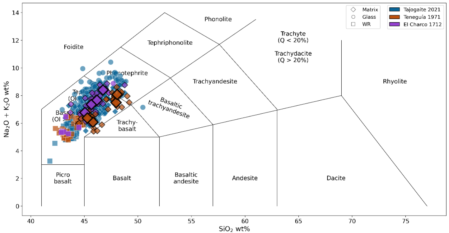
Supplementary Figure 12. TAS diagram. TAS diagram showing the matrix compositions studied in this work, compared with literature data. Large diamonds for Teneguía 1971 and El Charco 1712 represent the average matrix compositions based on 10 analyses from this study. Matrix data for Tajogaite 2021 Ubide et al. (2023) 15 . Whole-rock (WR) data for Tajogaite 2021 14–16 . WR data for El Charco 1712 27–30 and Teneguía 1971 22,24,27,30–32 were retrieved from the GEOROC database.
