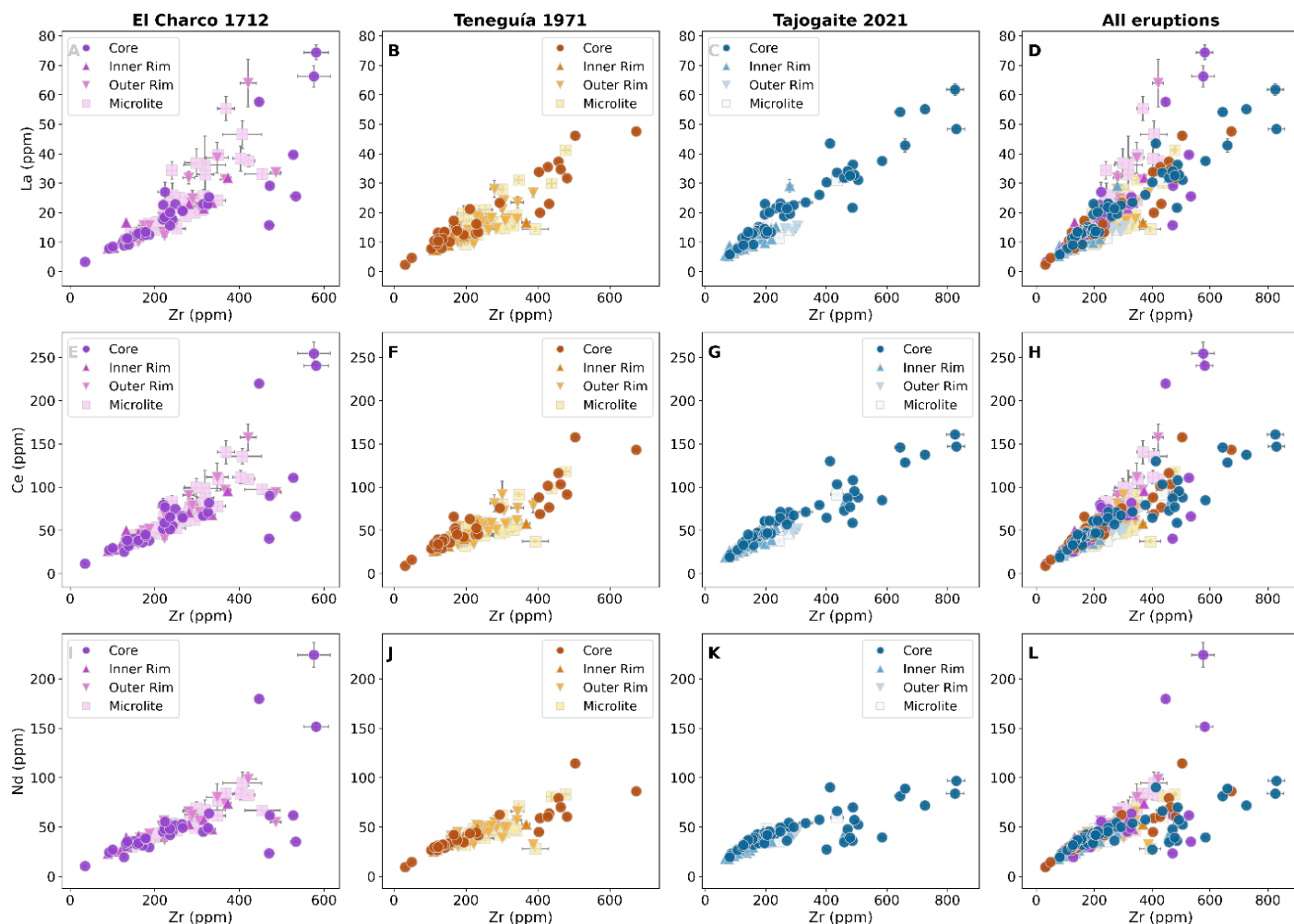
Supplementary Figure 7. Cpx incompatible TE composition (La, Ce, Nd). Clinopyroxene trace element bivariate plots of (A-D) La (E-H) Ce and (I-L) Nd vs Zr. Each column corresponds to a different eruption, as indicated by the column titles, with the final column showing data from all eruptions combined. Each symbol represents a different clinopyroxene textural position. Error bars indicate the internal 2SE analytical uncertainty.
