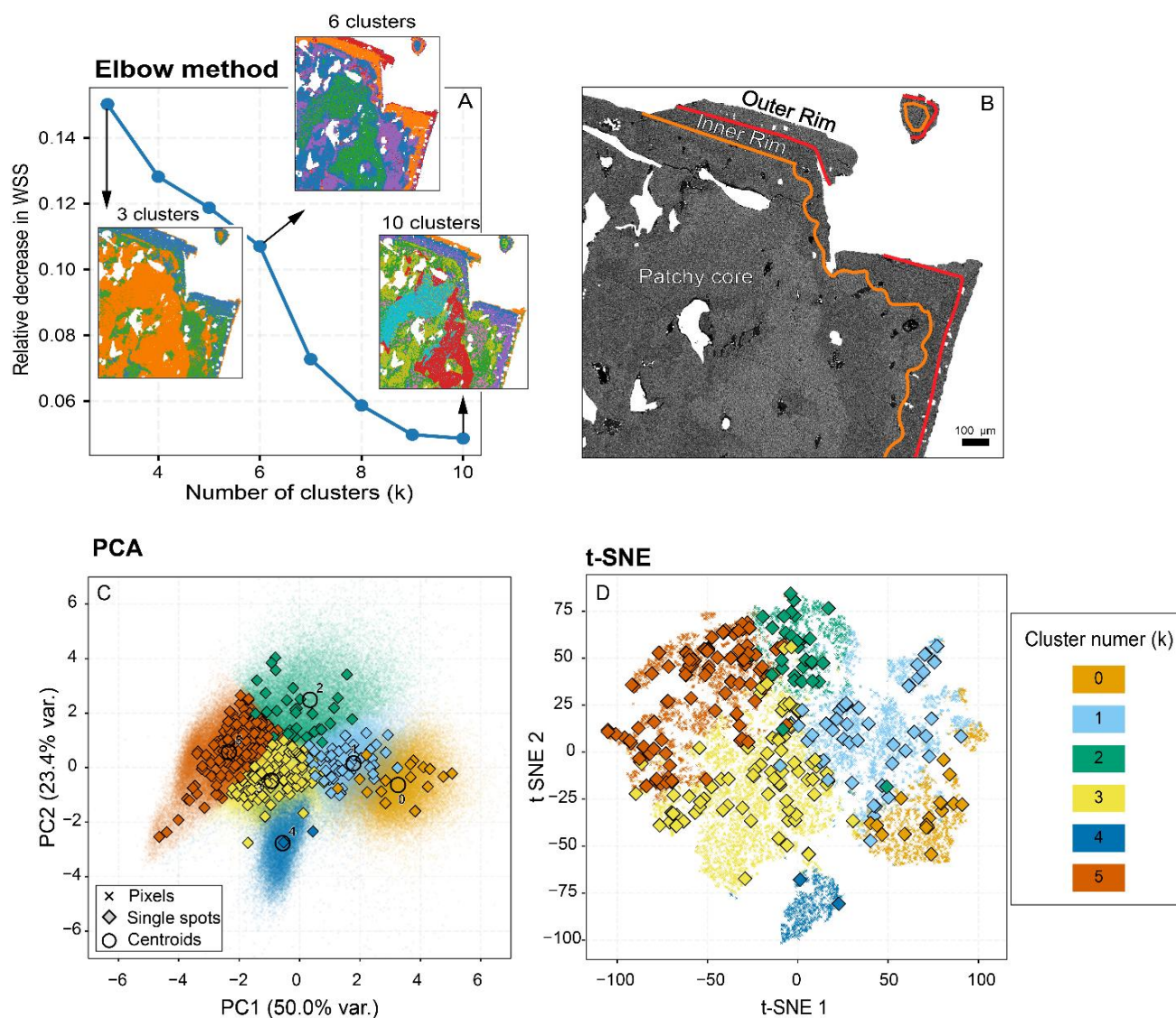
Supplementary Figure 24. Quantitative methods for selection of k . (A) Elbow method, showing the total variance within each cluster, expressed as within sum of squares (WSS), and cluster-coloured maps of a representative crystal for k = 3, 6 , and 10 . (B) Backscattered electron (BSE) image of the same crystal, highlighting texturally defined domains (outer rim, inner rim, and patchy core). (C) Single spots and pixel-data from maps in the principal component analysis (PCA) space. (D) t-SNE projection of the dataset coloured by cluster number, showing the formation of distinct compositional groups for both single spots and map pixel-data.
