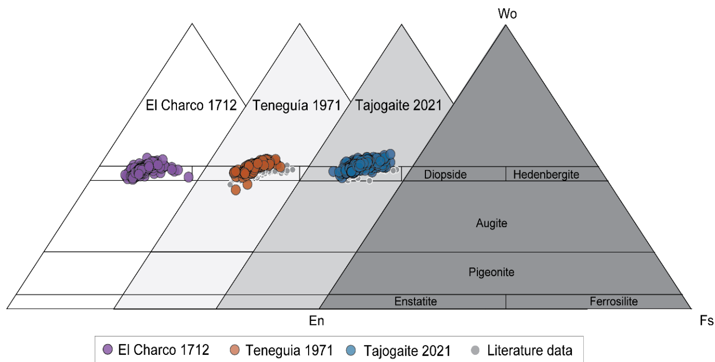
Supplementary Figure 1. Classification of Cpx. Composition of clinopyroxene crystals in the En-Fs-Wo ternary diagram. All compositions fall within the diopside field, with no differences between eruptions. Gray symbols represent clinopyroxene data from the literature 15,22–24 .
